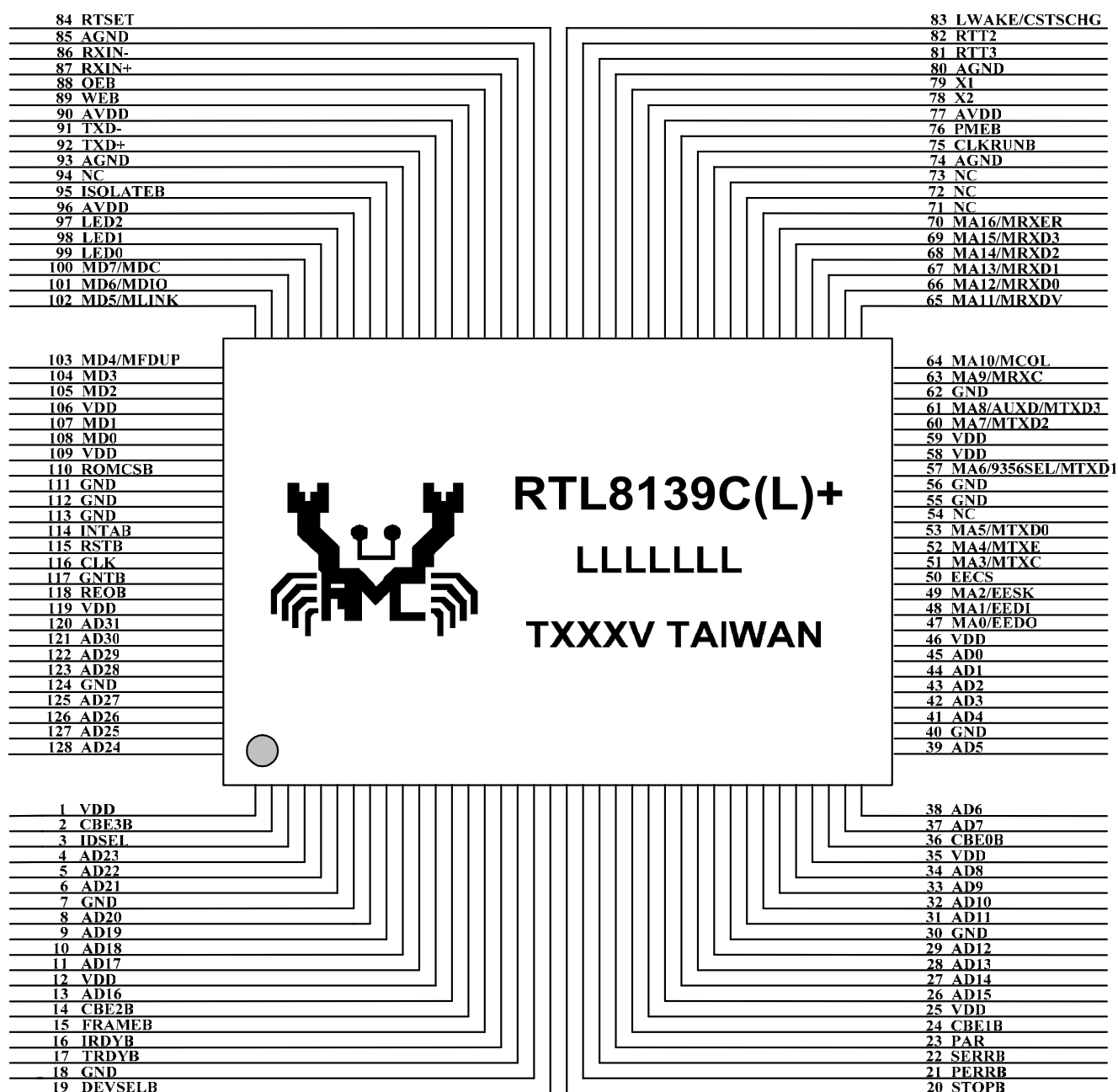
Figure 1. Pin Assignments (QFP & LQFP)
